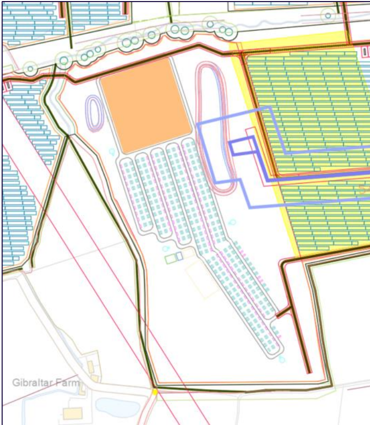
Figure 2.1: Illustrative Layout West BESS Site
